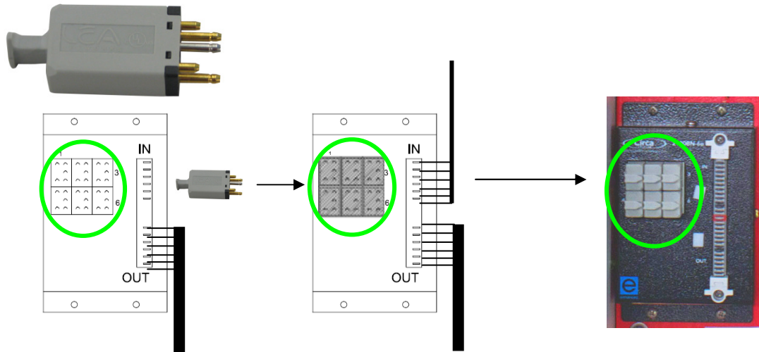
Fig. 20 Re-insertion of grey pass-through modules
