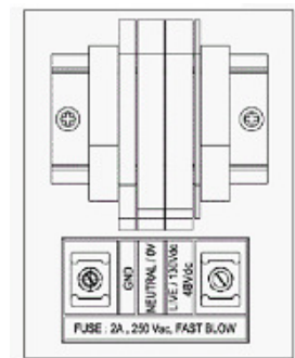
Fig. 1: Universal Power Input Terminal Block
