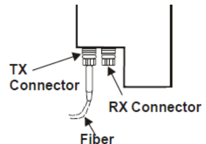
Fig 16: Fiber Connections
